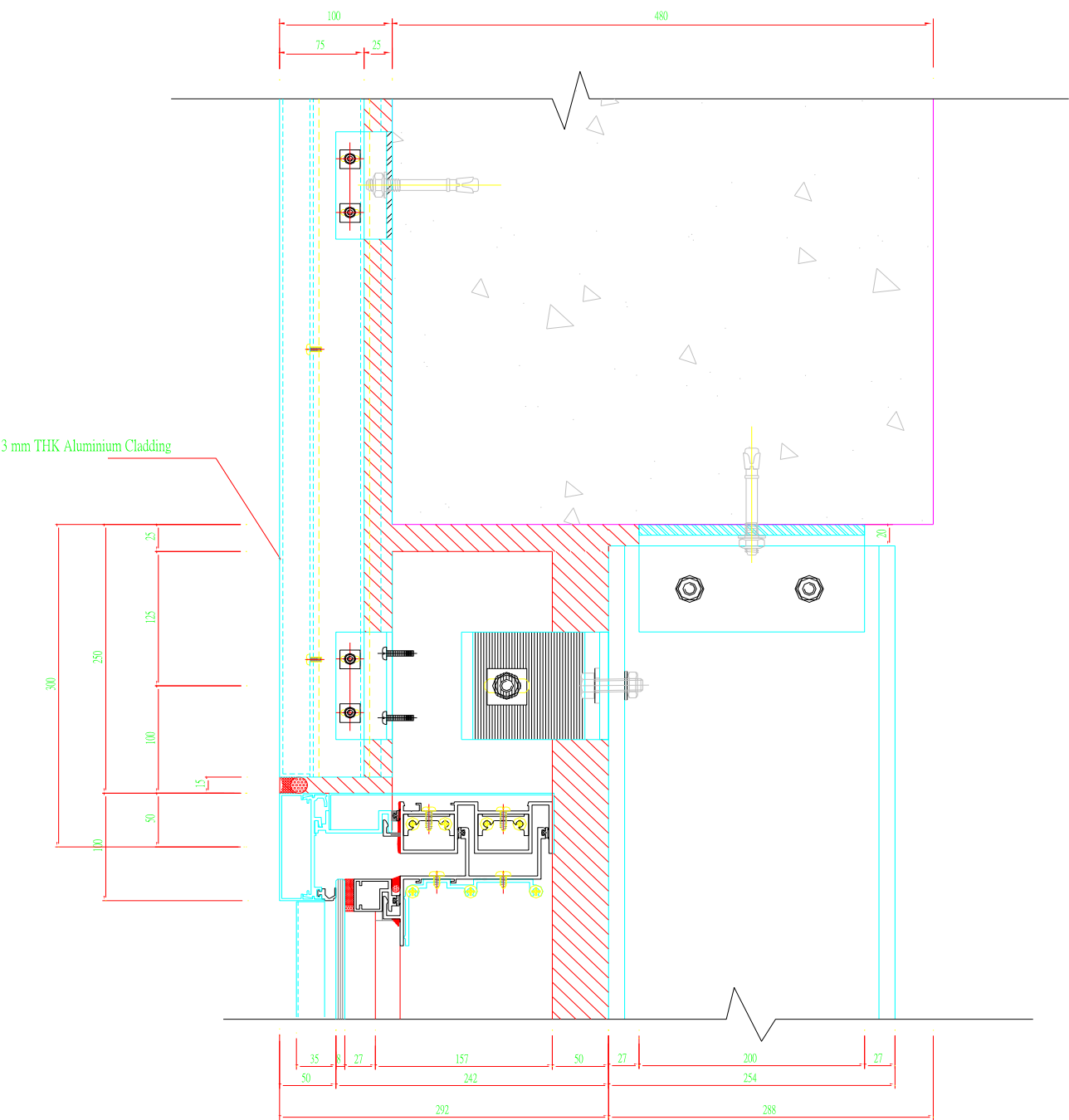
CROSS-SECTION A
