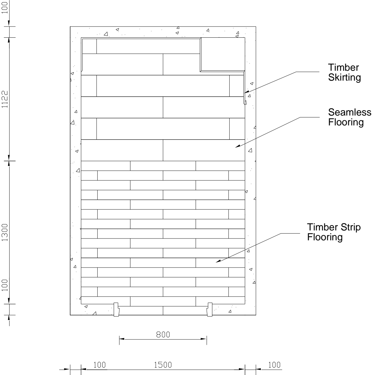
Layout Plan
