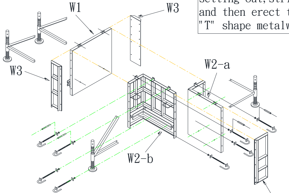
Isometric View
