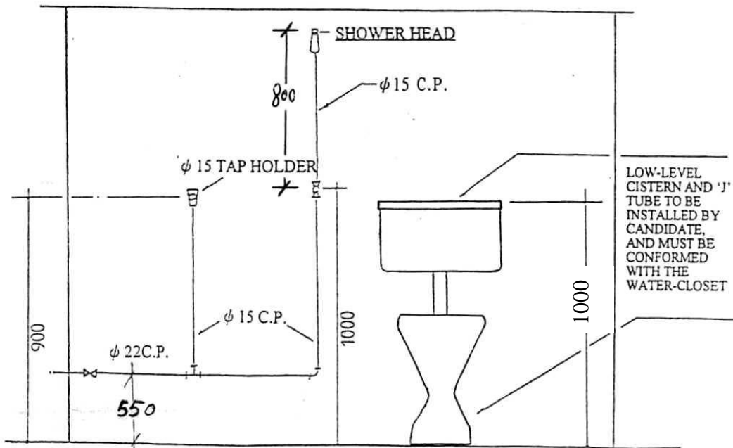
FRONT ELEVATION FROM 'A-A'
