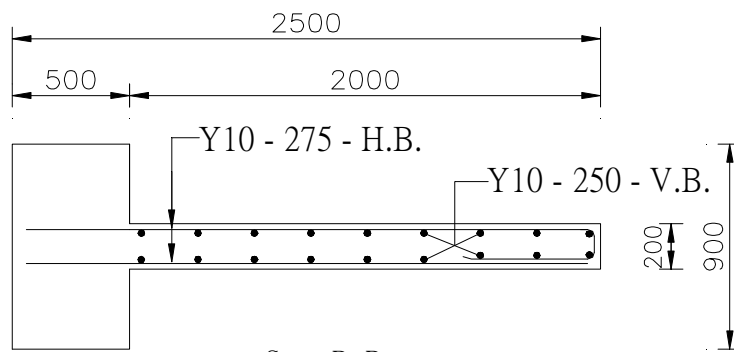
Sec B-B
