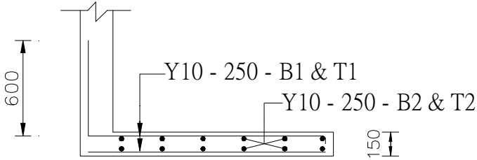
Sec C-C
