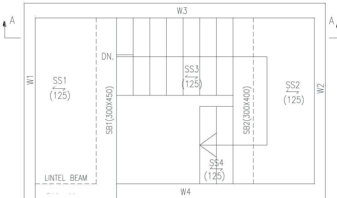
PLAN (1:30)
