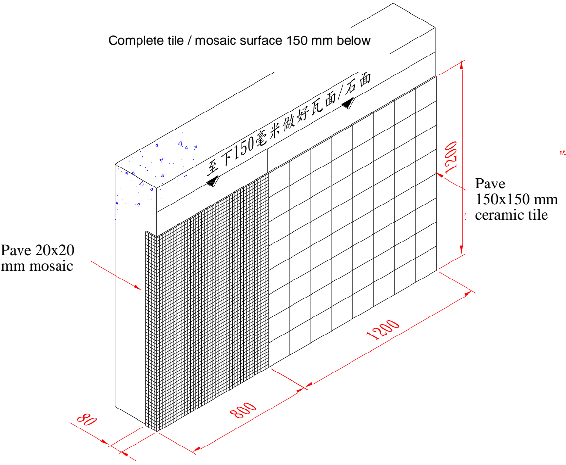
3-D Plan
