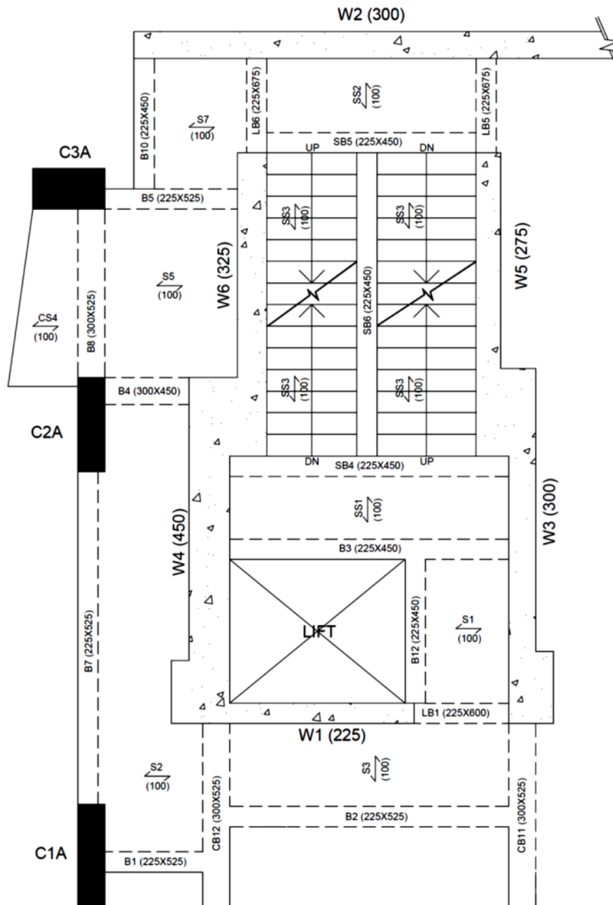
5/F TO 70/F FRAMING PLAN
