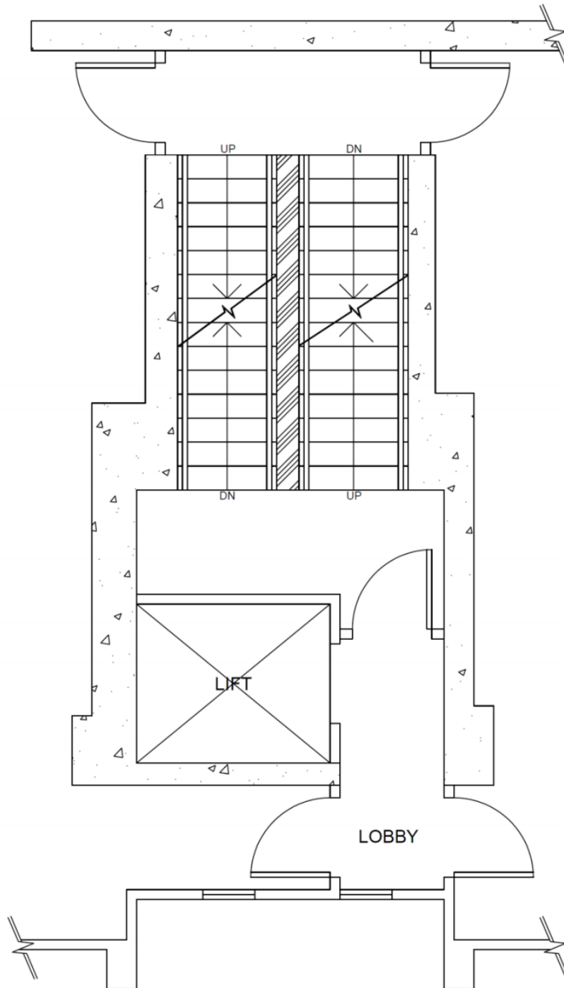
PART PLAN OF 35/F
