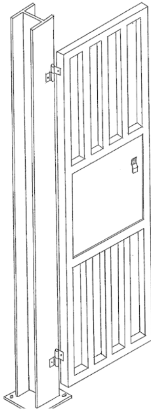
Trade Test Position (Synthetic Painting) Perspective Drawing
