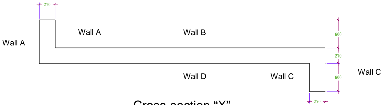
Cross-section "X"
