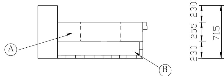
Front Elevation
