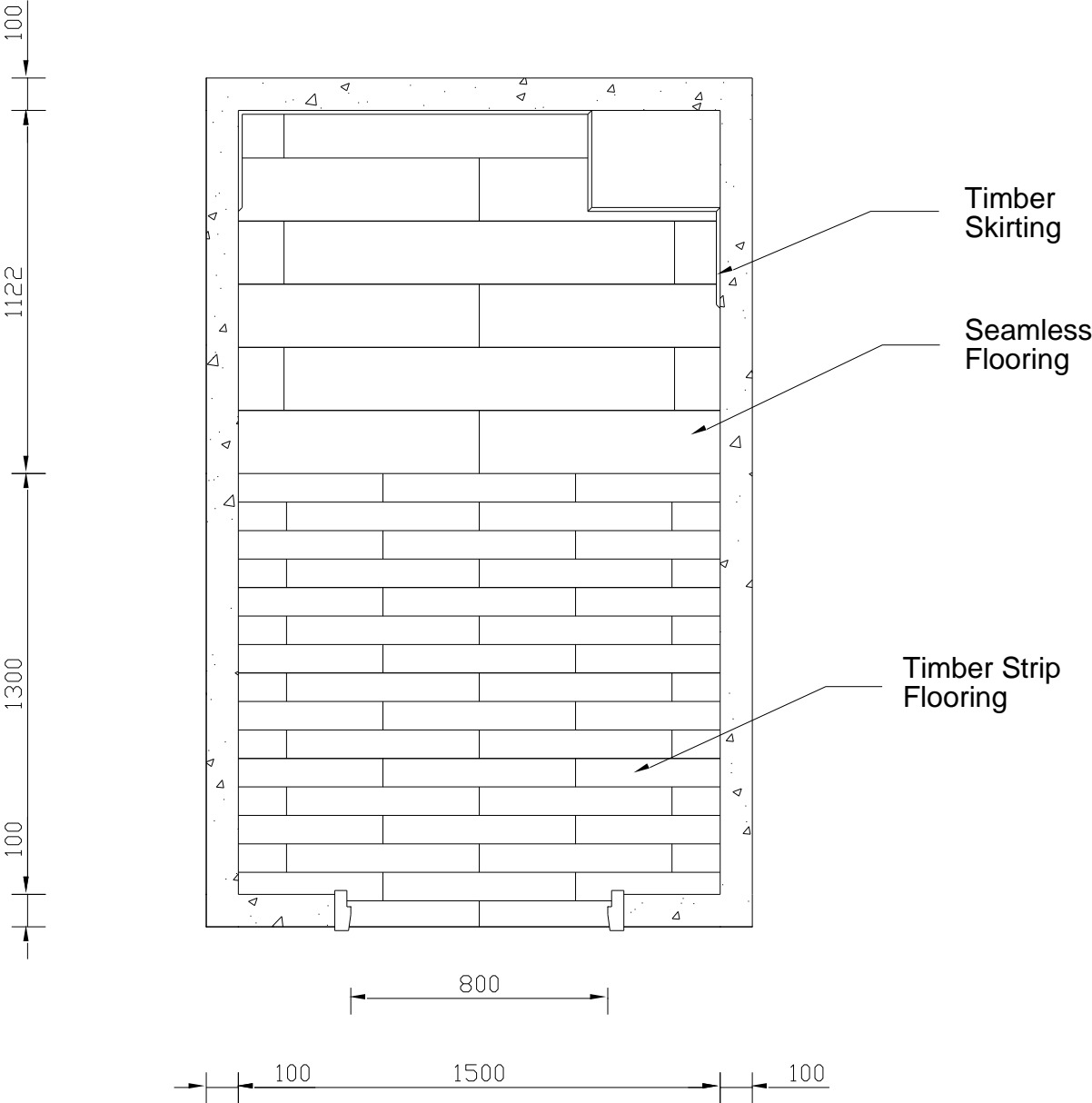
Layout Plan
