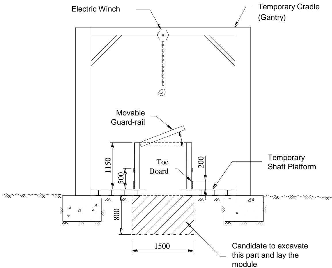
Cross-section
